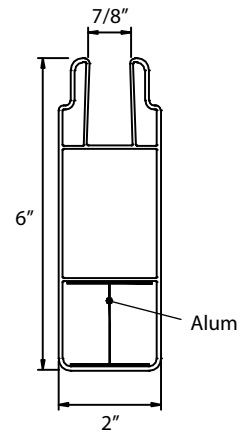
Side view of Alum insert
